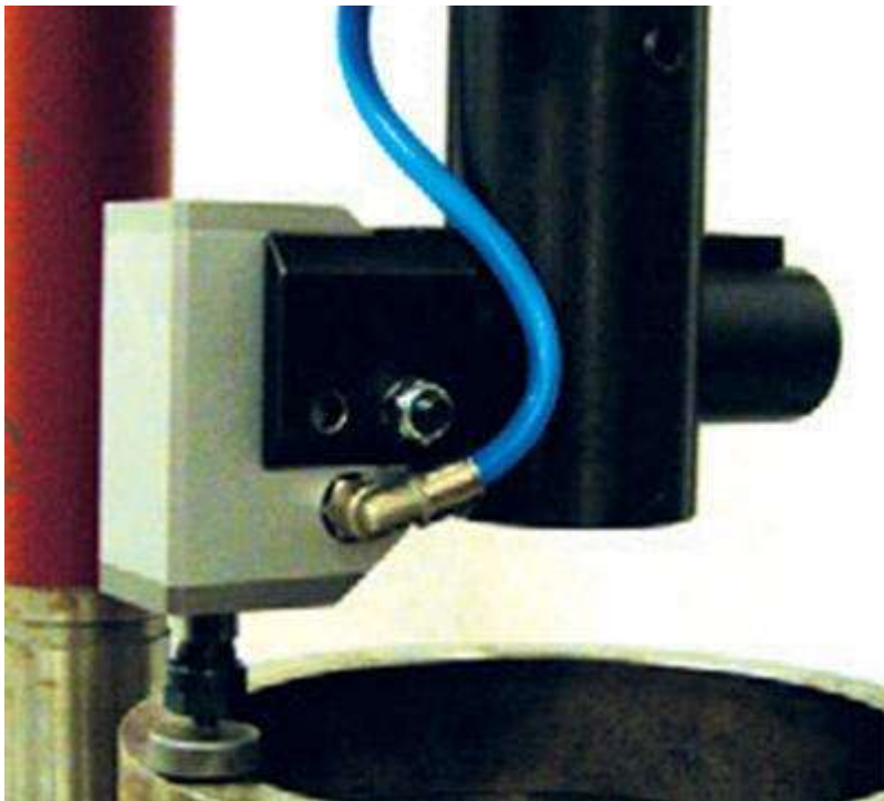
Model C - A portable, easy to mount, cutting, milling and grinding machine. Ideal for globe, safety and control valves
